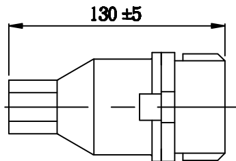
PLUG DETAIL
