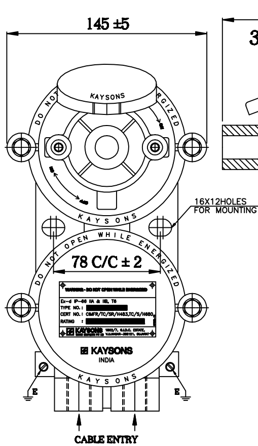
PLUG DETAIL
