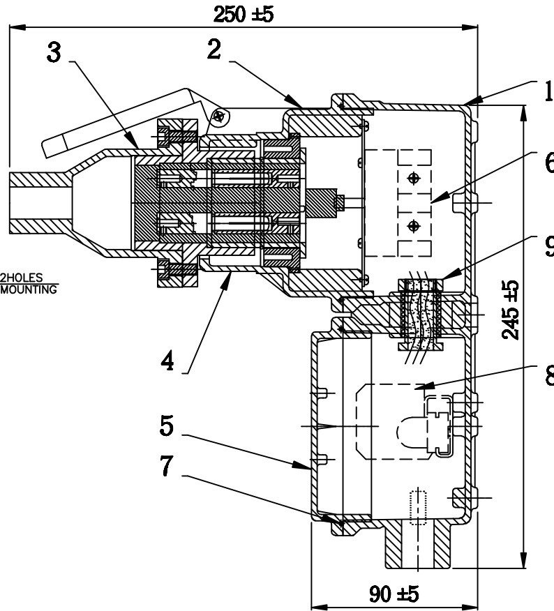
PLUG DETAIL
